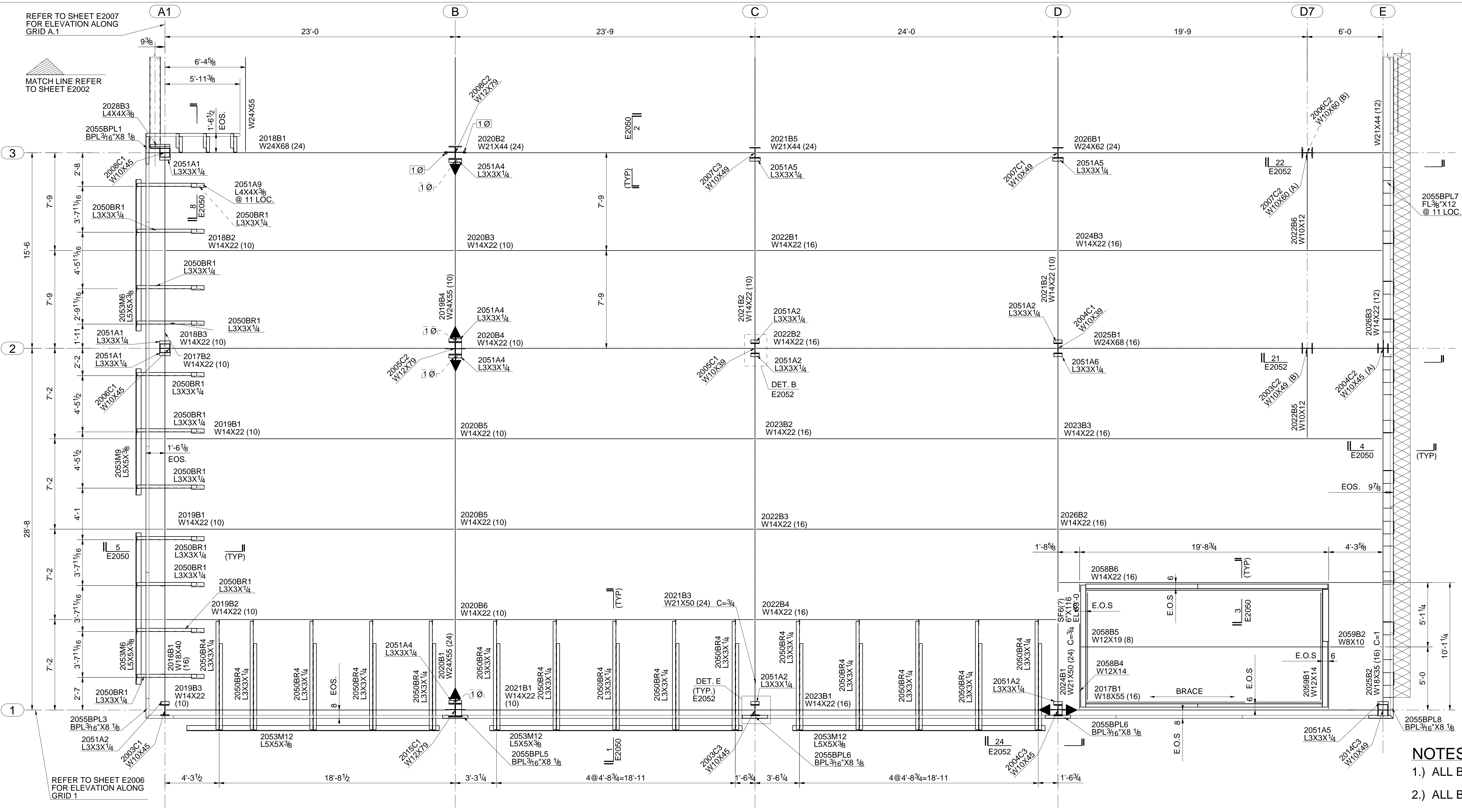
PARTIAL SECOND FLOOR FRAMING PLAN T.O.S EL = 79'-6 1/2" U.N.O
