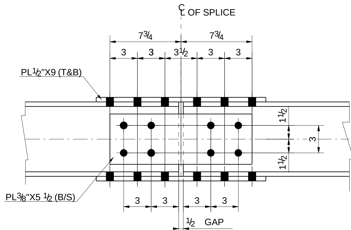
DETAIL J SPLICE DETAIL TOP & BOTTOM CHORD
