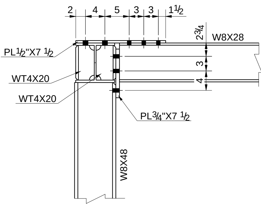
4 SECTION E25005 (TYP@W8X48 POST)
