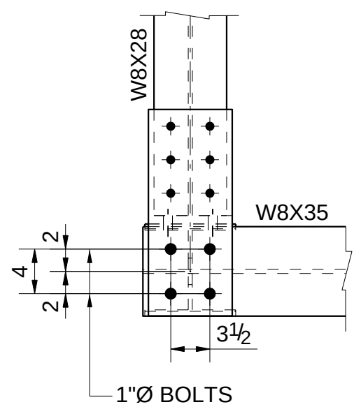
DETAIL E E25005
