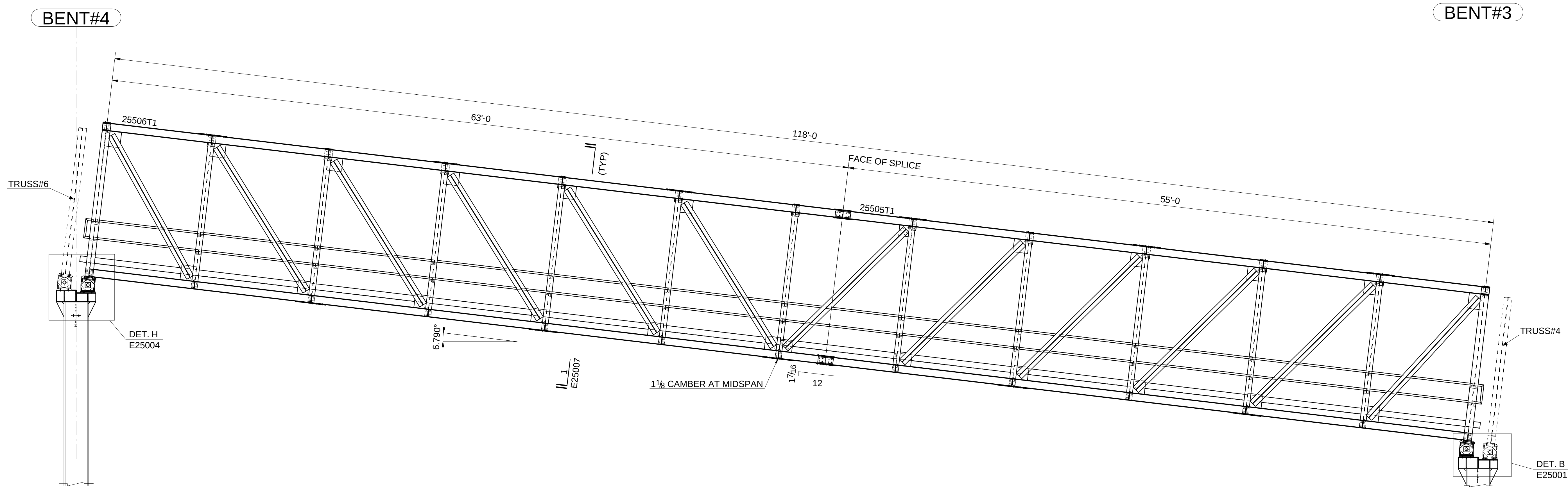
ELEVATION @ TRUSS #5 LOOKING EAST
