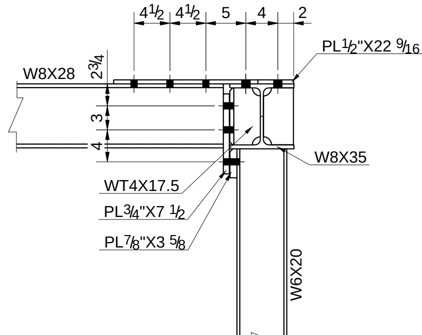
6 SECTION E25005 (TYP@W6X20 POST)
