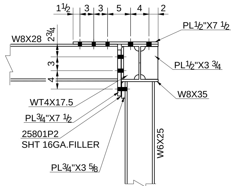
5 SECTION E25005 (TYP@W6X25 POST)
